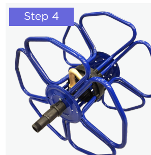
Step 4: Push second rotary drum (A) onto the other side of the drum joiner (H).
