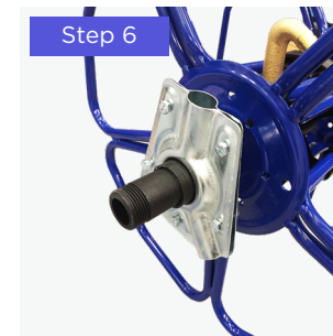
Step 6: Loosely assemble clamps (J) using the M4 bolts & nuts (L), so that the support frames (B) and axle (C) can slide into them. Position them on the shoulders of the spacers (F).
